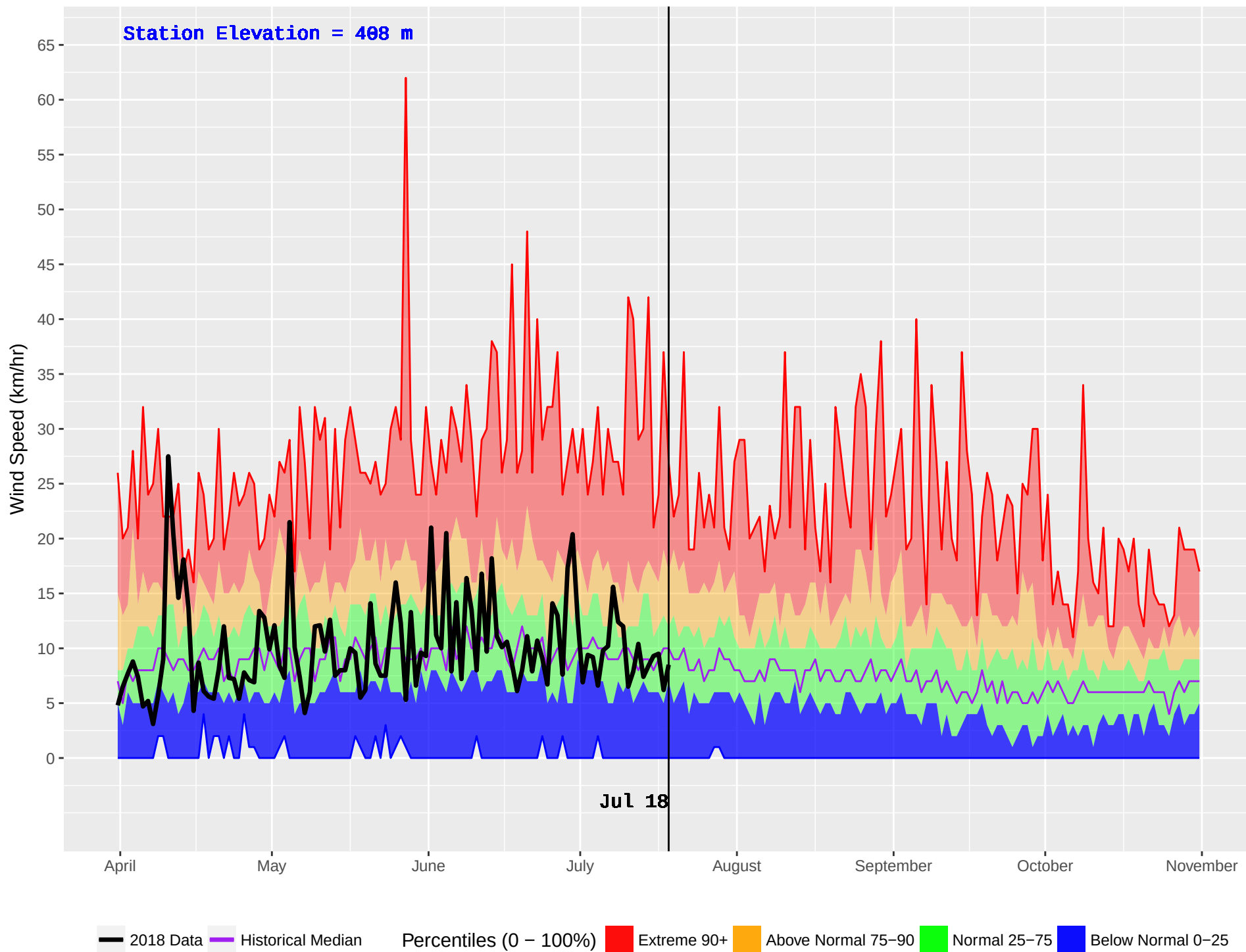
LILLOOET (280) : Historical (1977–2016) and Current (2018) Daily Wind Speed
